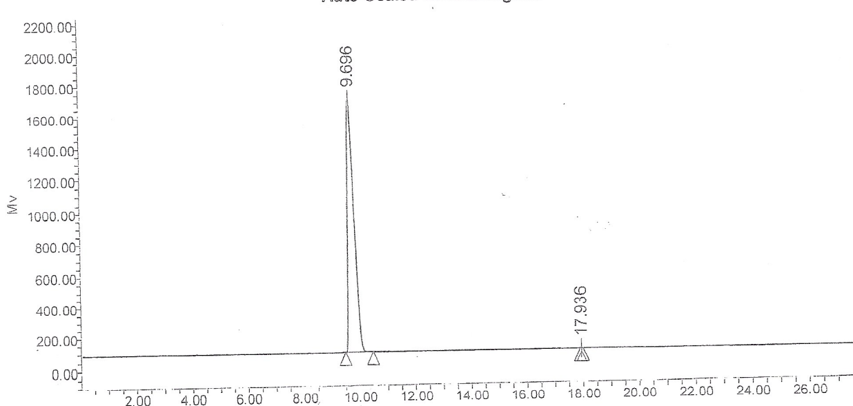
Auto-Scaled Chromatogram
